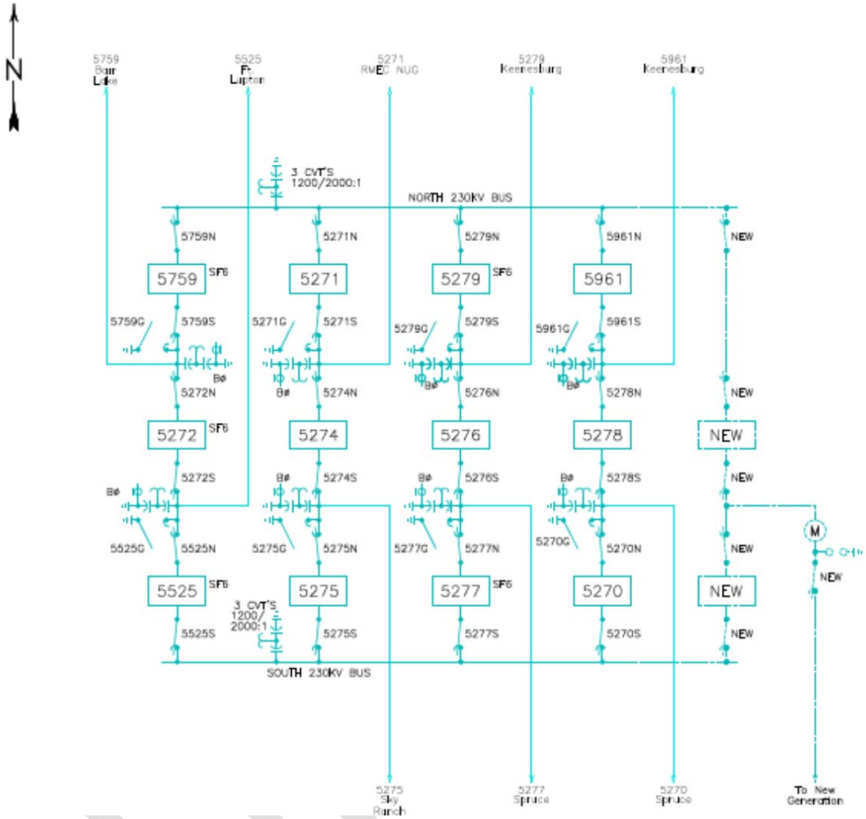
Figure 2: GI-2016-24 Interconnection to 230 kV Bus in Green Valley Station
