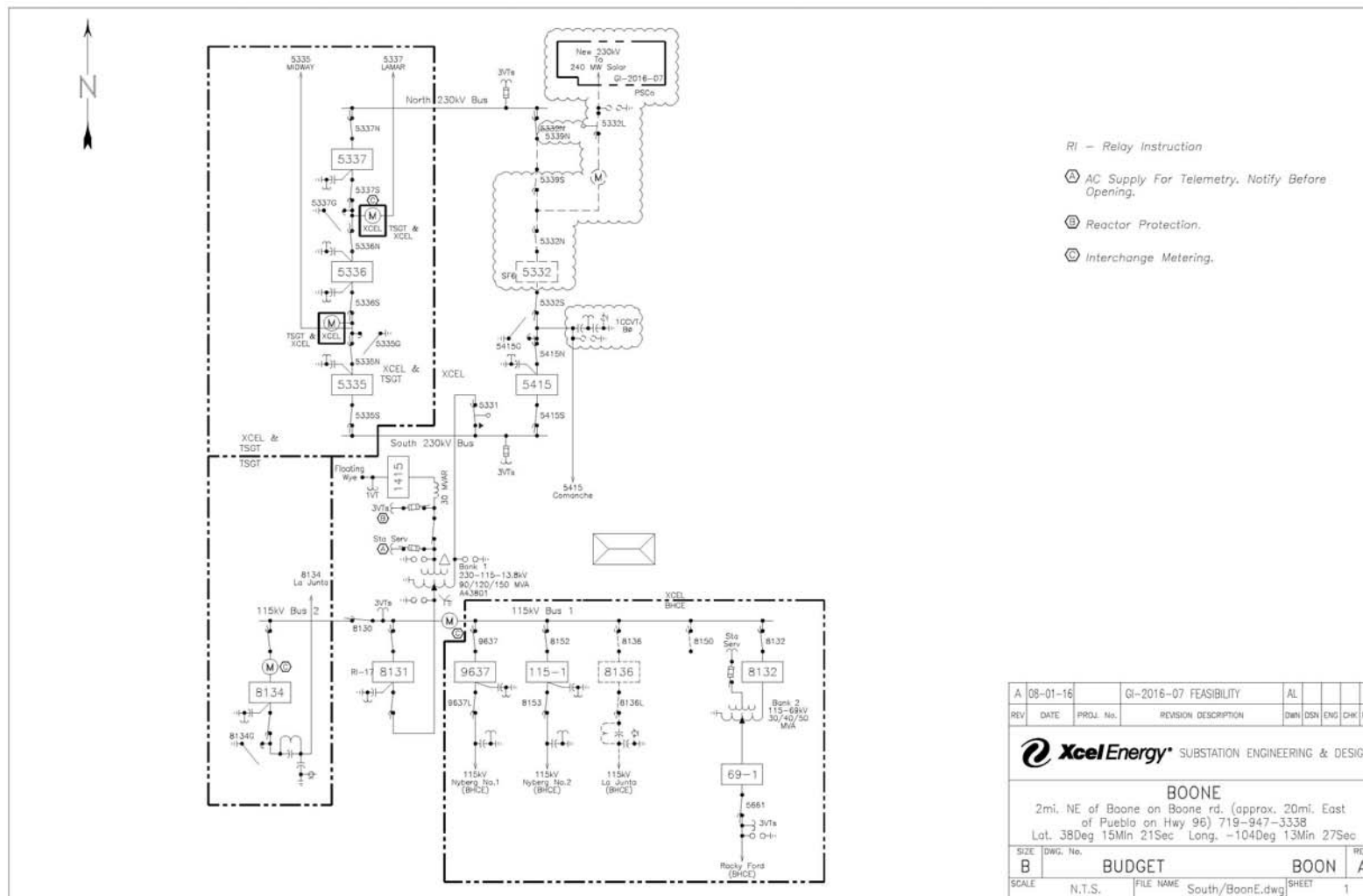
Figure 2 – GI-2016-7 Conceptual One-Line Diagram of the POI
